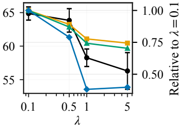
CIFAR-10
