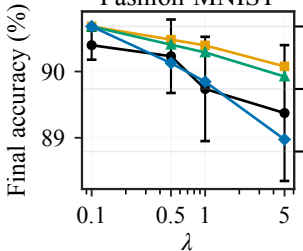
Fashion-MNIST
